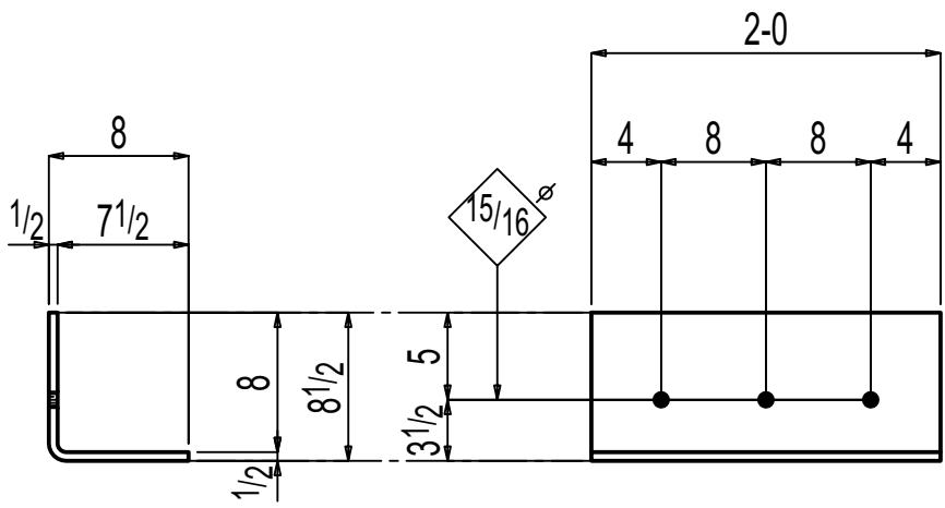
ONE BENT PLATE F-08.03M1
