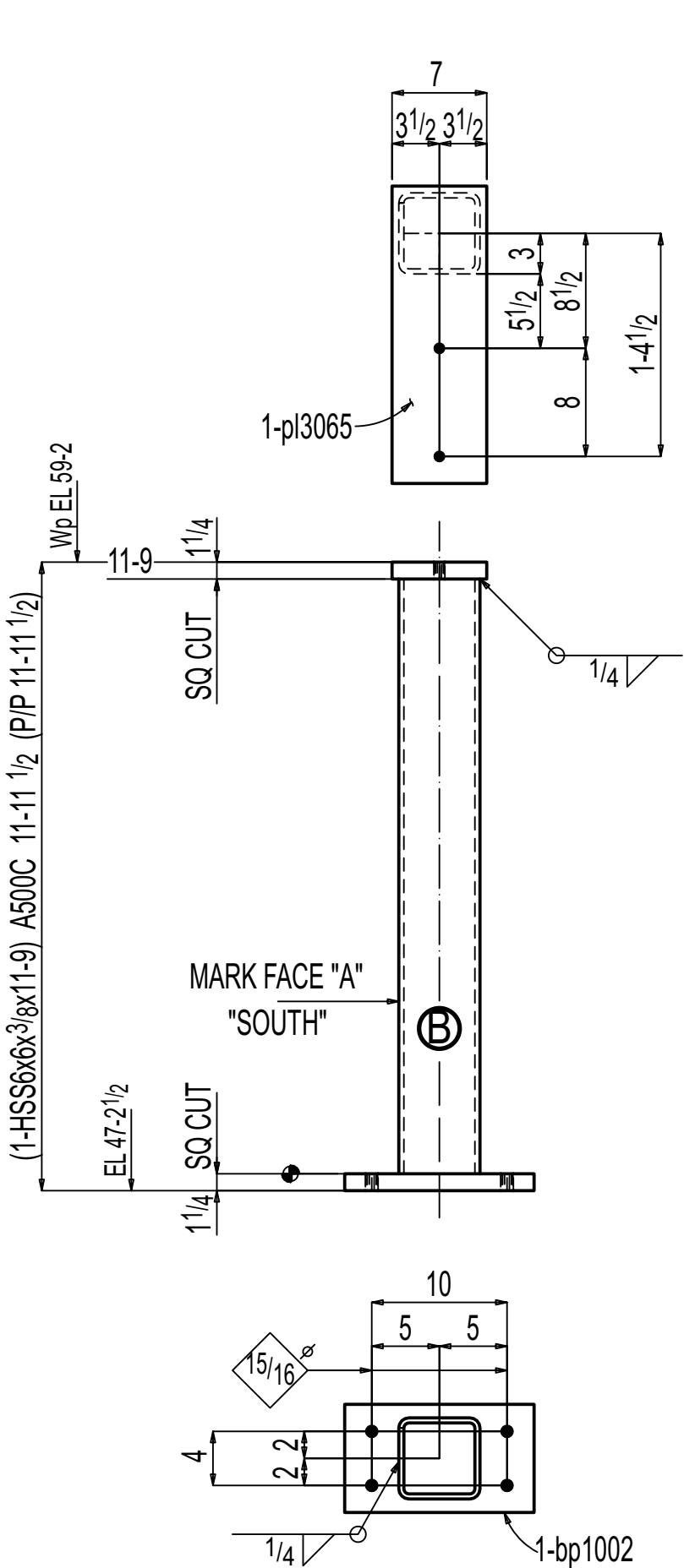
ONE COLUMN F-08.00C1
