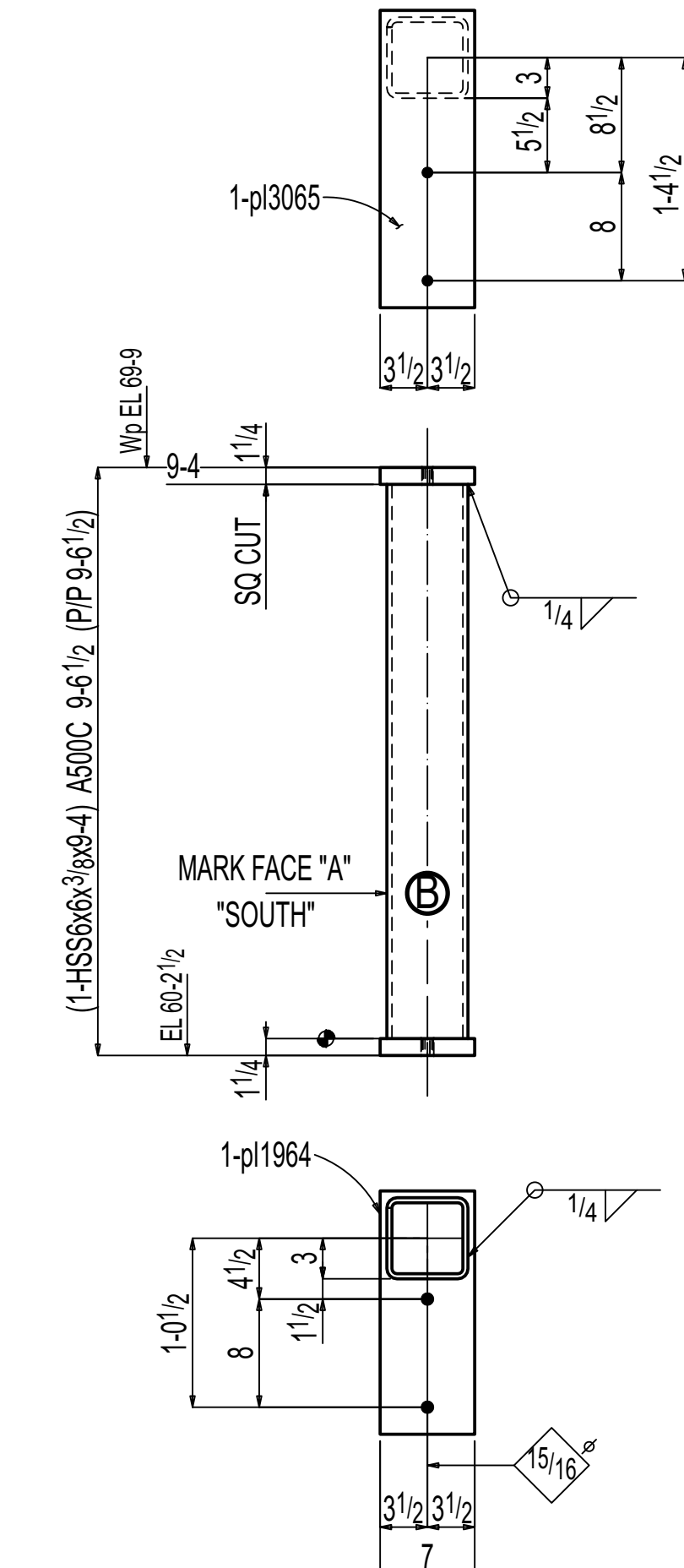
ONE COLUMN F-08.00C2
