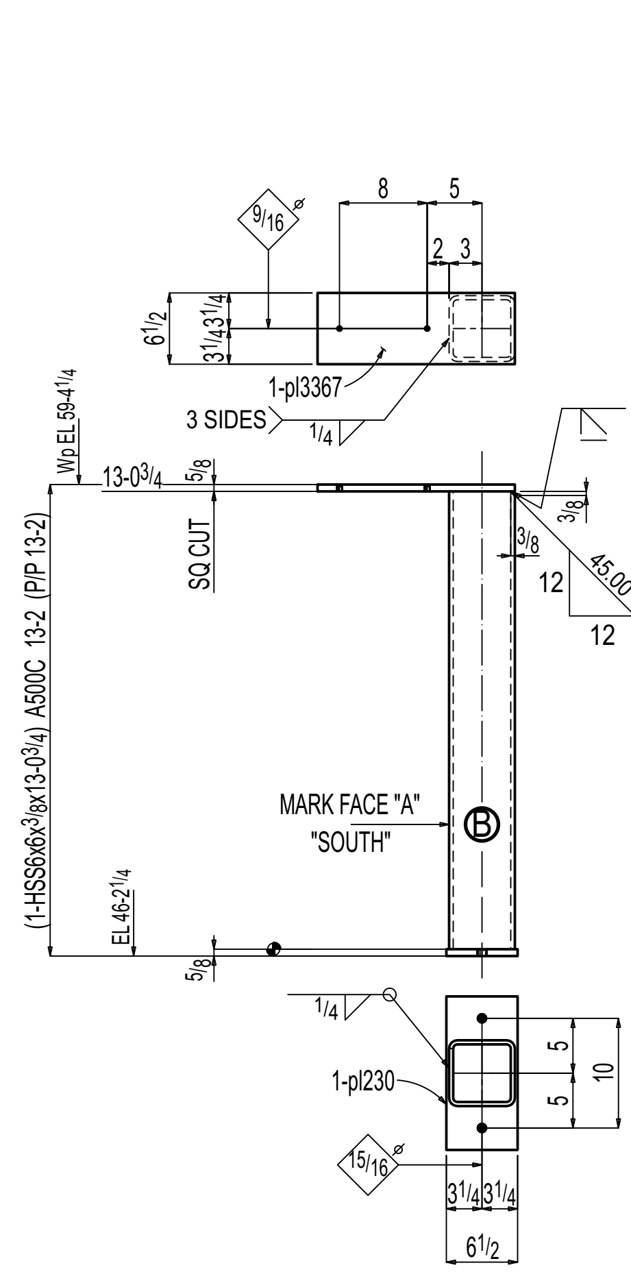
ONE COLUMN F-08.00C3
